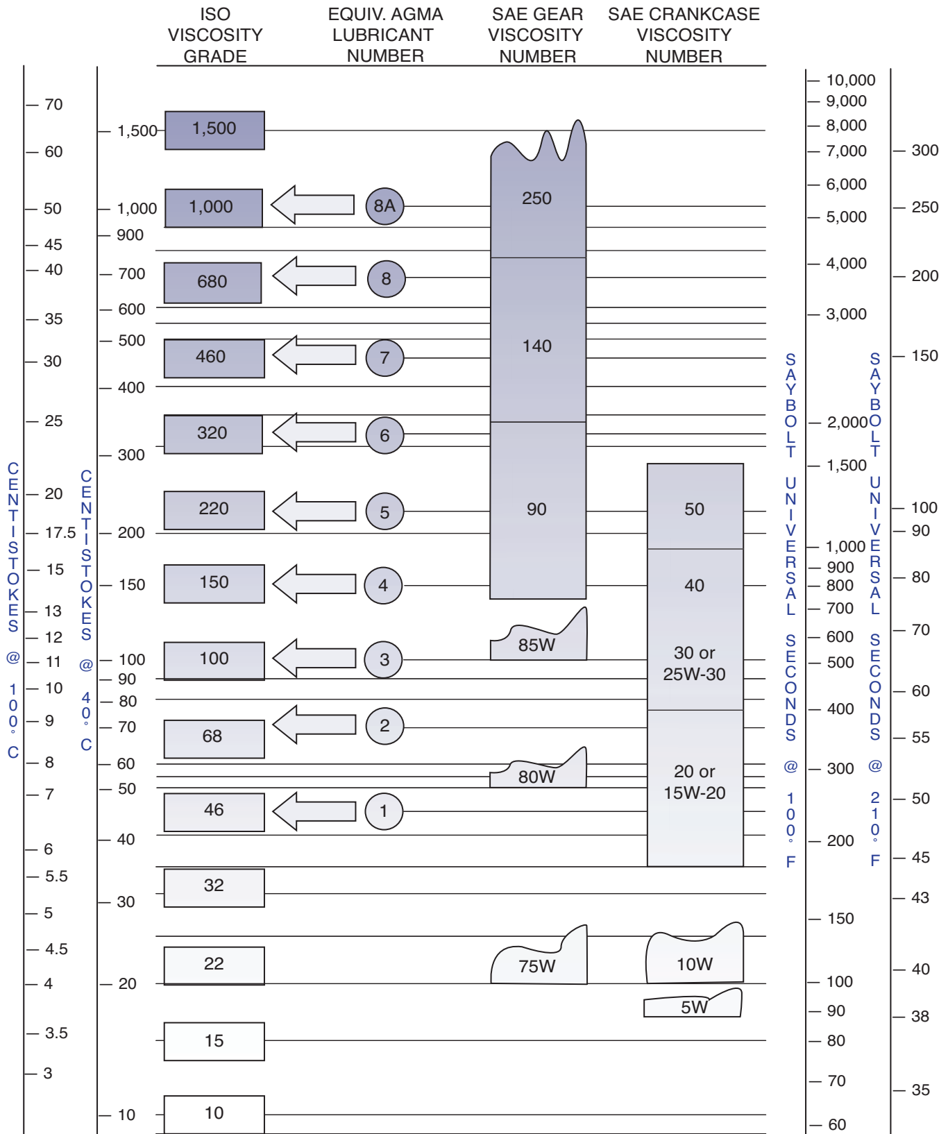
VISCOSITIES AT VARIOUS TEMPERATURES ASSUME 95 VI OILS
